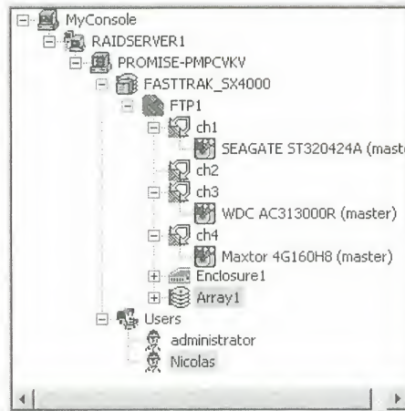
Figure 4-2. An example of a RAID system in Tree View.
