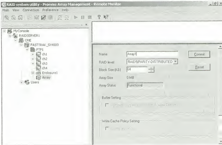
Figure 3-6. New Array information window.
