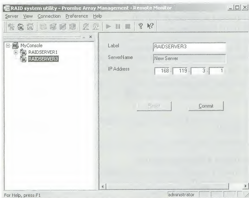
Figure 5-2. Changing a RAID server's Label and IP address.
