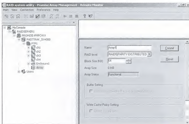
Figure 5-14. New Array information window.
