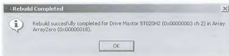
Figure 5-21. Rebuild Successful.
