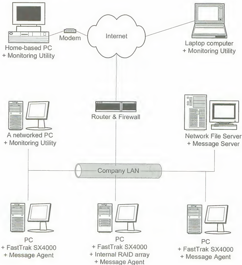
Figure 1-1. LAN and Internet connections.
