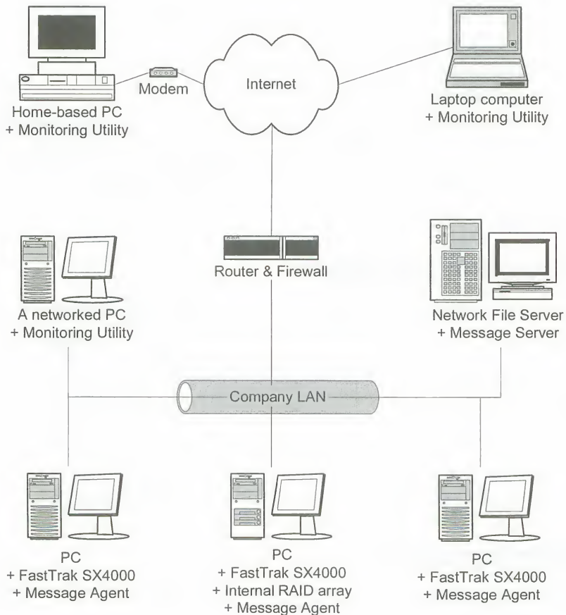
Figure 2-1. Networked RAID has many installation options.
