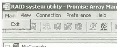
Figure 4-7. Main Menu.
