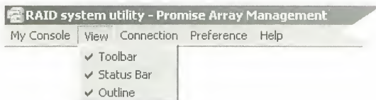
Figure 4-8. View Menu.
