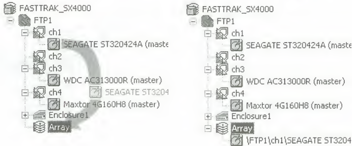
Figure 5-15. Drag and drop unassigned drive icons onto the array icon.
