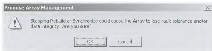
Figure 5-22. Stop Warning.
