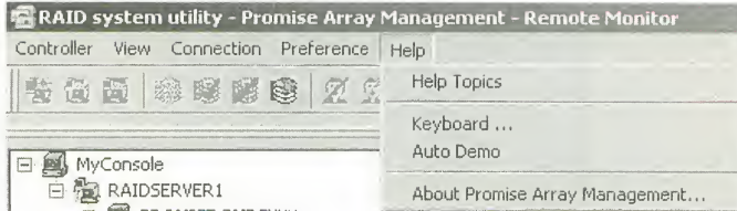
Figure 4-11. Help Menu.
